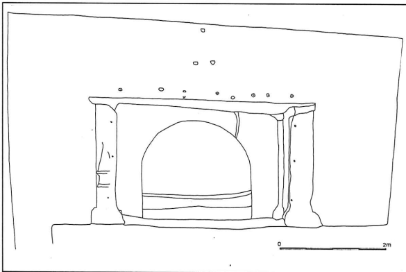
8. East elevation of the interior of Tomb 825.
