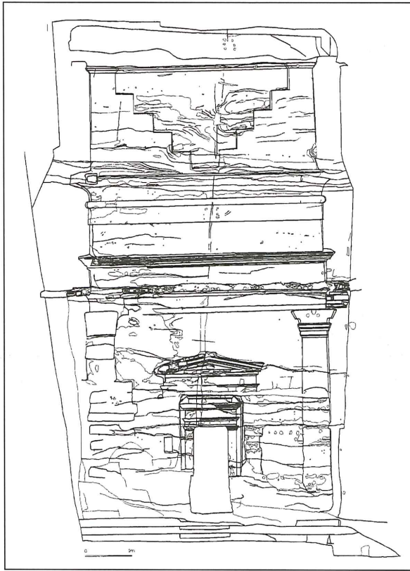
5. Façade of Tomb 825.
