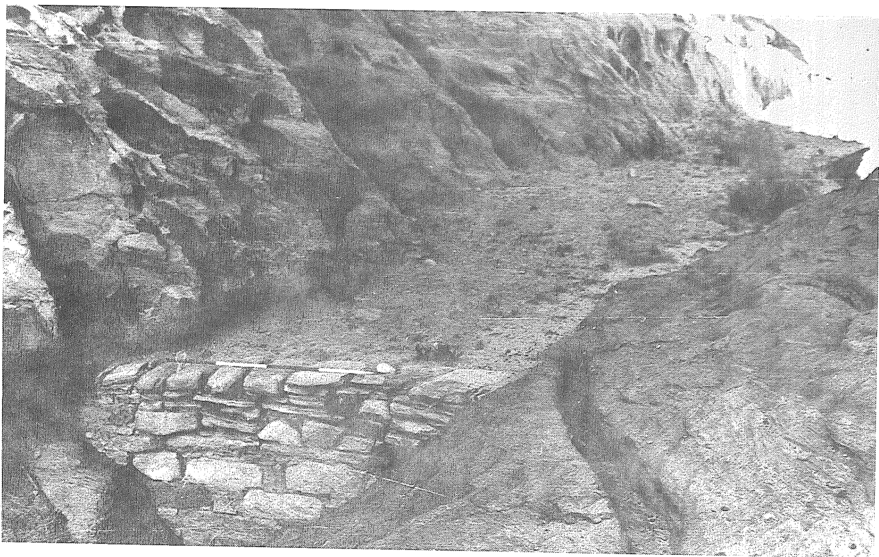
Pl. XXXVI, 1: Tell el Kharaza dam and water channels
