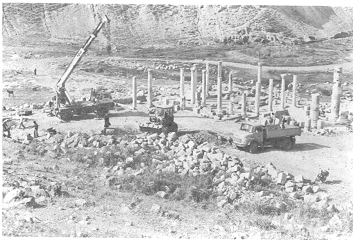
Pl. LXXVII, 2: Department of Antiquities technicians repairing and re-erecting a column of the sanctuary of the Civic Complex Church on its original base.
