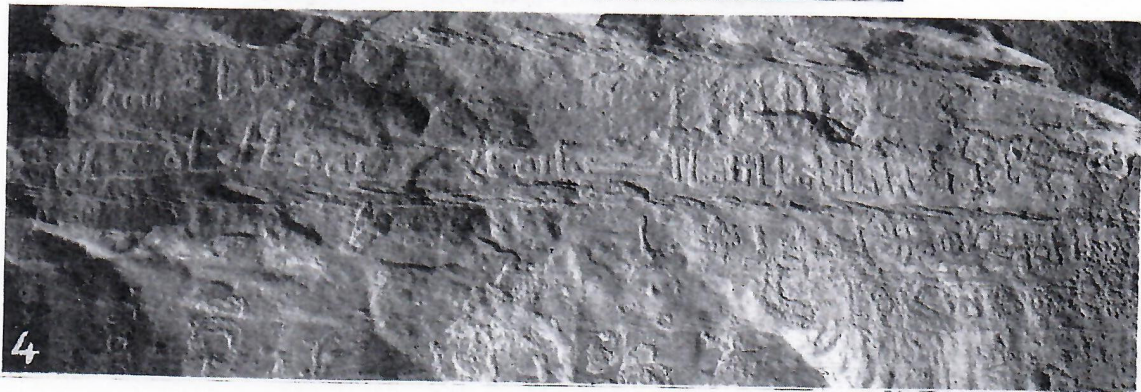
Kufic Inscriptions
