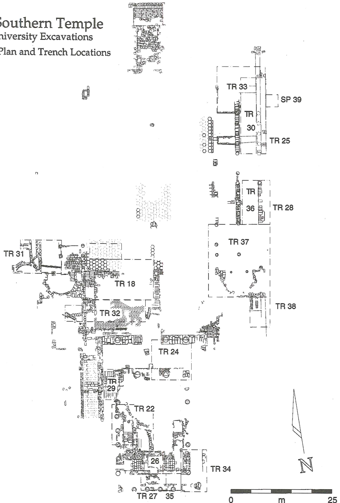
3. 1996 Site plan with trenches. (D. Pitney, L. Traxler, P. Zimmerman).
