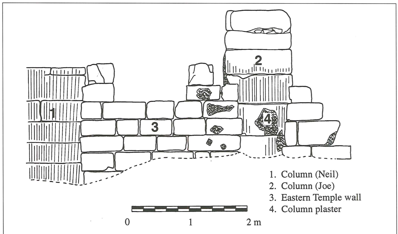
16. Drawing of the Trench 34, Locus 14 (Field drawing by L. D. Bestock, Drafted by A. H. Bedewy).
